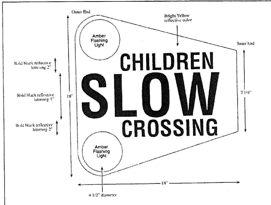
Figure 1. Signal Arm.
